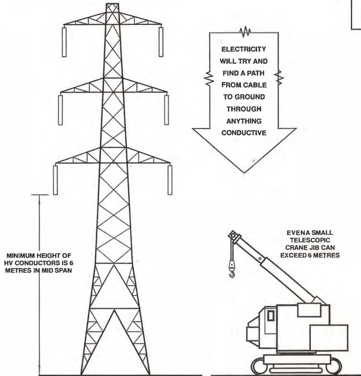
TYPICAL 275Kv AND 400Kv HIGH VOLTAGE TRANSMISSION LINES ON STEEL TOWERS
